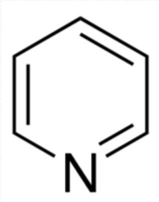
Pyridine
