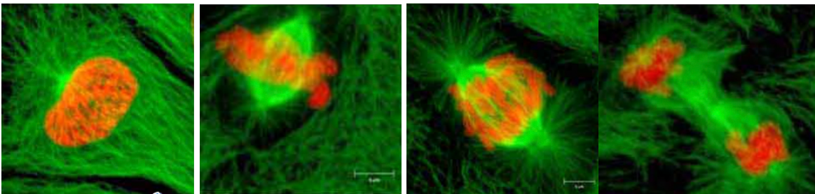
Prophase
